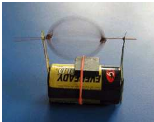
(Simple Motor)
