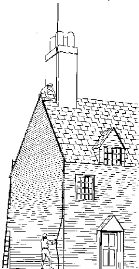
Lightning rod on a chimney stack
